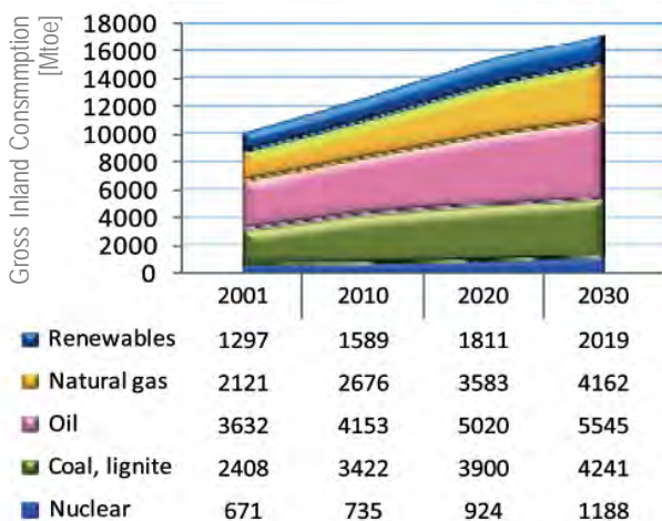
Global energy mix and CO 2 emissions
