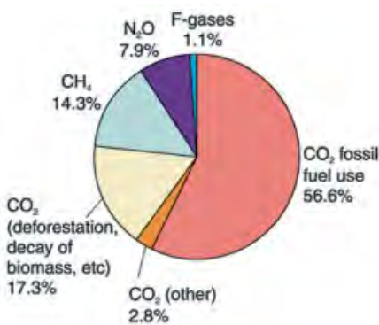
Global anthropogenic GHG emissions
